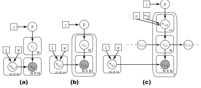
Figure 1: Graphical model of (a)IRM (Eqs.2-5), (b)“tIRM” (Eqs.7-10), and (c)dIRM (Eqs.11-15). Circle nodes denote variables, square nodes are constants and shaded nodes indicate observations.
