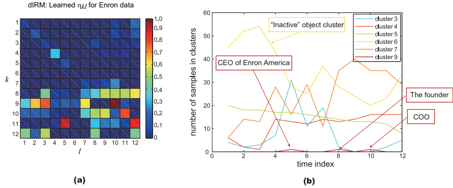
Figure 4: (a): Example of estimated \eta_{k,l} for Enron dataset using dIRM. (b): Number of items belonging to clusters at each time step for Enron dataset using dIRM.
