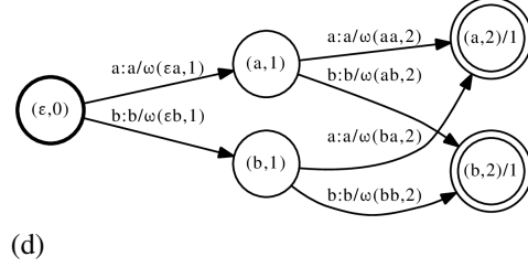
Figure 2: (a) Efficient computation of the key terms of the structured gradient for the rational loss. For each transition e \in E_{\mathbf{z}, s} , we denote its origin by \underline{e} , destination by \bar{e} and weight by \omega(e) . (b) Illustration of the WFA \bar{\mathcal{Y}} for \Delta = \{a, b\} and l = 3 . (c) Illustration of the WFA \mathcal{Y}_i representing string dac . (d) Illustration of WFA \mathcal{A} for q = 2 , alphabet \Delta = \{a, b\} and string length l = 2 . For example, the transition from state (a, 1) to state (b, 2) has the label b and weight \omega(ab, 2) = e^{\mathbf{w} \cdot \psi(x_i, ab, 2)} .
