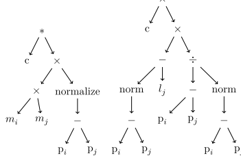
Figure 8: Learned force expression for FALL (left) and SPRING (right)
