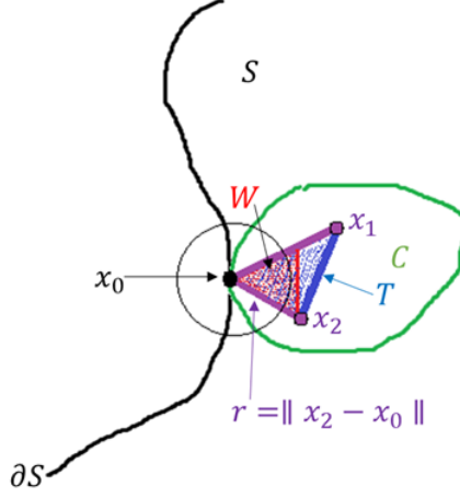
Figure 6: The convex set C , the simplex T , and the simplex W in two dimensions. The illustrated ball has radius less than r . In this Figure, r = \|x_2 - x_0\| .
