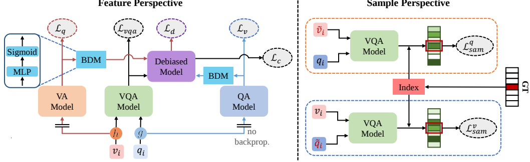
Figure 2: Overview of our D-VQA method. Our method alleviates the biases from feature and sample perspectives. From the feature perspective, we introduce question-to-answer, vision-to-answer, and debiased branches to help reduce the negative biases. BDM is the bias detection module. Note that \mathcal{L}_d does not optimise the VQA model. From the sample perspective, we construct two types of negative samples to assist the model’s training. (v_i, q_i) denotes a positive sample, while (\tilde{v}_i, q_i) and (v_i, \tilde{q}_i) are negative samples. GT is the ground-truth answer of (v_i, q_i) . h and g are the feature extractors.
