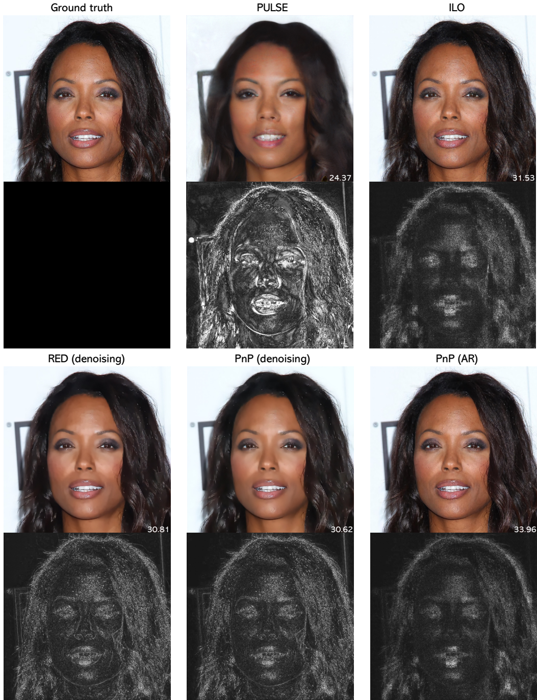
Figure 9: Visual comparison between PnP/RED and two methods using generative models, when applied to the CelebA HQ dataset at 10% sampling ratio. The error residuals to relative to the ground truth images were amplified 7\times and showed in grayscale for better visualization. Note the similarity between the RED and PnP solutions. PnP (AR) leads to sharper images, comparable to those obtained by ILO with StyleGAN2. This highlights the benefit of using pre-trained AR operators.
