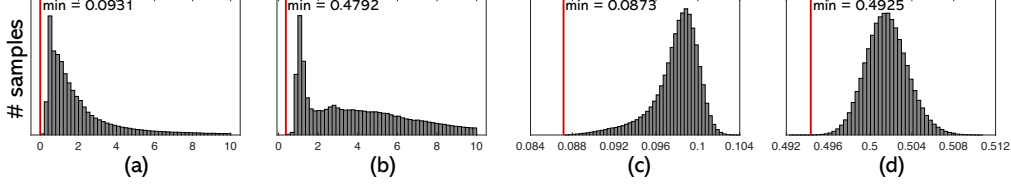
Figure 2: Empirical evaluation of the S-REC constant \mu > 0 for the measurement operators \mathbf{A} used in our simulations. We tested both the AWGN denoisers and the AR operators by randomly sampling from their image spaces \text{Im}(\mathbf{D}) . The x -axis is the value of \|\mathbf{A}\mathbf{x} - \mathbf{A}\mathbf{y}\|_2^2 / \|\mathbf{x} - \mathbf{y}\|_2^2 . (a) and (b) show the histograms for the radially sub-sampled MRI matrices at 10% and 50% sampling ratios, respectively. (c) and (d) show the histograms for the random Gaussian matrices for the same two sampling ratios. As expected, one can observe the increase in \mu for the higher sampling ratio of 50%.
