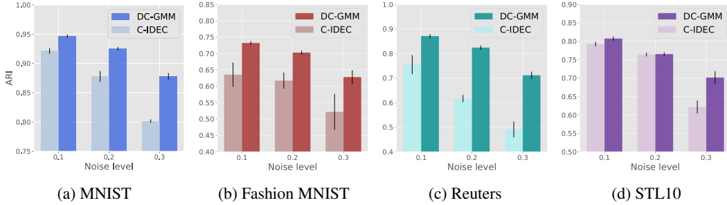
Figure 3: Comparison of clustering performance of our proposed DC-GMM model and the strongest baseline C-IDEC on four different data sets with noisy labels. ARI is used as evaluation metric.
