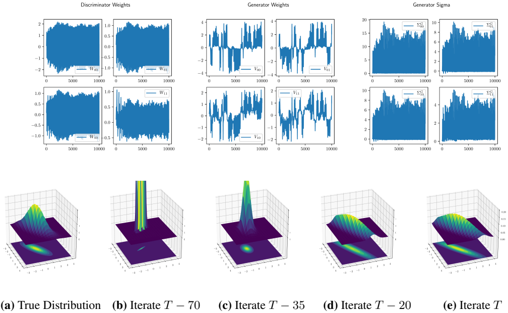
Figure H.7: GD for covariance learning of a two-dimensional gaussian without weight clipping using a batch size of 50. Comparison of true distribution and distribution of generator at various points at the end of training.
