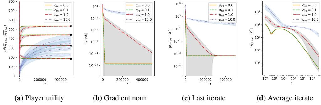
Figure H.3: Different levels of relative noise using adaptive DualX. The \mathcal{O}(1/T) rate for the average iterate (last plot) is kept even when the noise level is increased to \sigma_{\text{rel}} = 1.0 .
