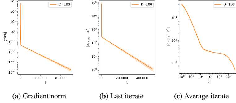
Figure H.6: DualX in a higher dimensional kelly auction ( N = 100 ). Let the total resources be Q = 1000 , cost of bidding be Z = 100 and the marginal utility gains be G = (6.001, 6.002, \dots, 6.1) (see Section 6 for exact definitions). Since the problem size is out of scope for Mathematica to provide a numerical solution we computed the optimal point using adaptive DualX for 2.5 million full steps with fine-tuned diameter in a deterministic setting. The experiment is then subsequently performed with \sigma_{\text{rel}} = 0.1 for 500 000 iterations.
