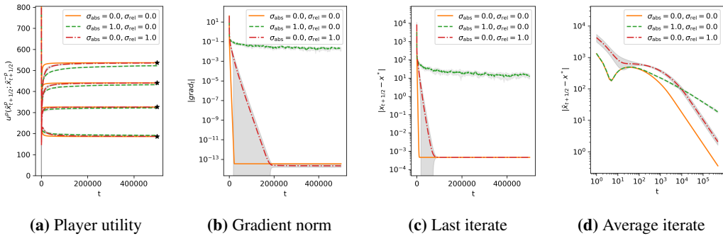
Figure H.2: Relative noise compared with absolute noise using adaptive DualX. We observe the deterioration of the rate for the average iterate for absolute noise in contrast with relative noise.
