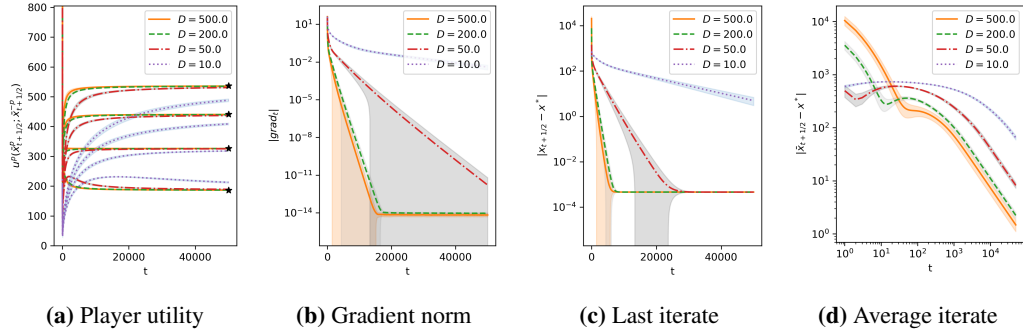
Figure H.5: We compare the effect of the diameter choice for adaptive DualX on a Kelly auction with \sigma_{\text{rel}} = 0.2 . We can observe the \mathcal{O}(1/T) average iterate rate for the whole spectrum of diameters but we note that the choice of diameter still has practical impact on convergence time. The fastest convergence is achieved with the highest diameter but note that the method did not converge for D = 1000 which we have excluded to keep the plots readable.
