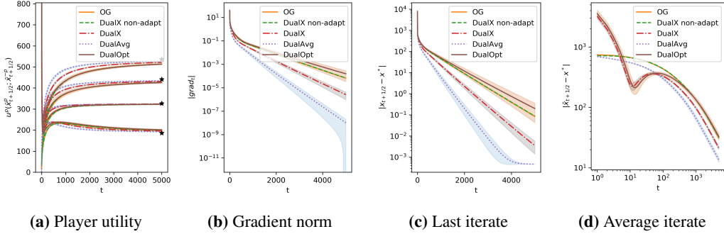
Figure H.1: Comparing methods with \sigma_{\text{rel}} = 0.1 .
