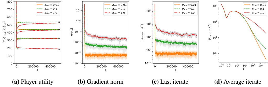
Figure H.4: Different levels of absolute noise using adaptive DualX. In contrast with relative noise increasing the absolute noise clearly worsens the slope for the average iterate (last plot) indicating a rate of \mathcal{O}(1/\sqrt{T}) .
