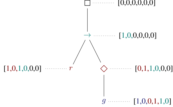
Figure 2: Example tree positional encoding for the LTL request pattern \Box(r \rightarrow \Diamond g) .
