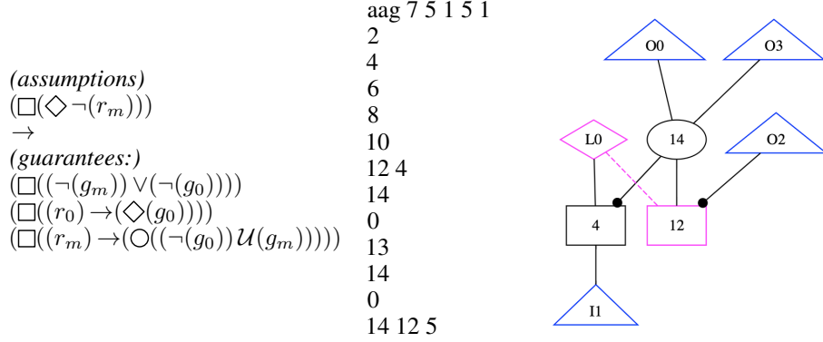
Figure 7: The specification (left), the predicted AIGER circuit (middle) and the visualization of the circuit (right) for a prioritizing arbiter.
