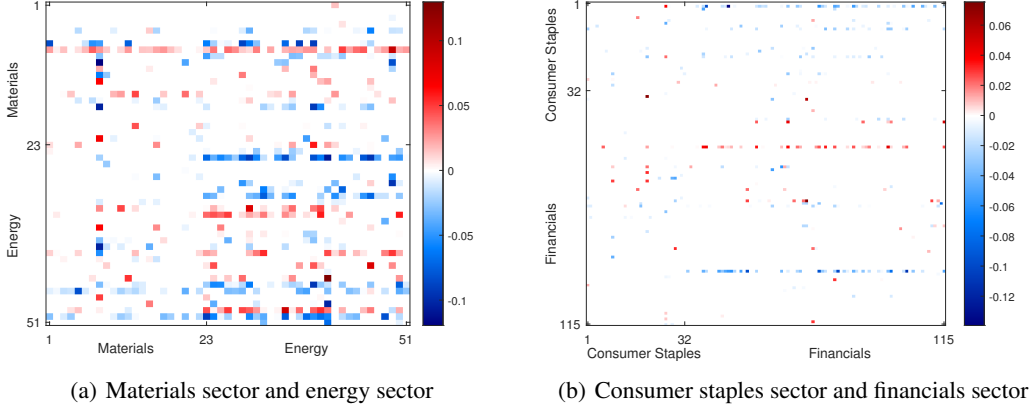
Figure 4: Sparsity patterns of the transition matrix \hat{\Gamma} estimated by FNSL.
