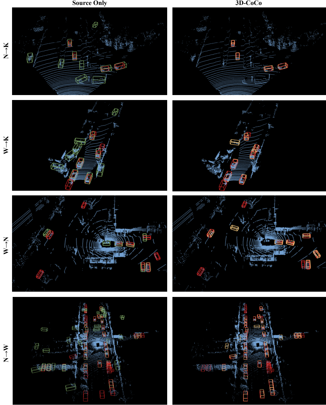
Figure 5: Qualitative results on four adaptation tasks. N : nuScenes; K : KITTI; W : Waymo. Red : Ground-truth; Green : Predictions by the Source Only model; Yellow : Predictions by 3D-CoCo. Obviously, the predictions of 3D-CoCo align better with the ground-truth bounding boxes.
