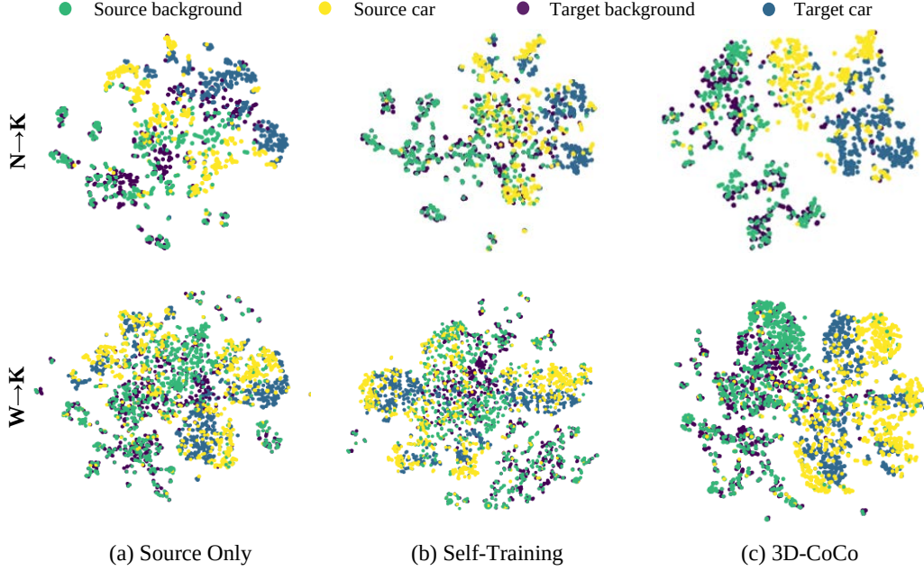
Figure 3: The t-SNE visualization of sample features. (a) The source only model is trained without any adaptation technique. (b) The self-training method applies the pseudo-labels on target data for re-training, but it fails to align the distribution of features from the source and target domains without any access to the source data. (c) The proposed 3D-CoCo framework leverages both labeled source data and unlabeled target data for co-training, which obviously enhances the intra-class compactness and encourages inter-class separability in the feature space. N : nuScenes; K : KITTI; W : Waymo.
