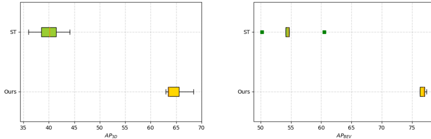
Figure 4: The box-plot on AP 3D (Left) and AP BEV (Right) for 3D-CoCo and self-training (ST).
