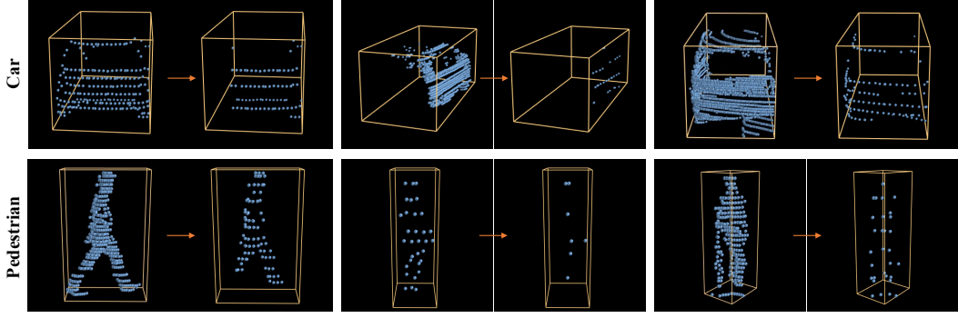
Figure 2: The visualization of mined hard examples for the categories of Car and Pedestrian.
