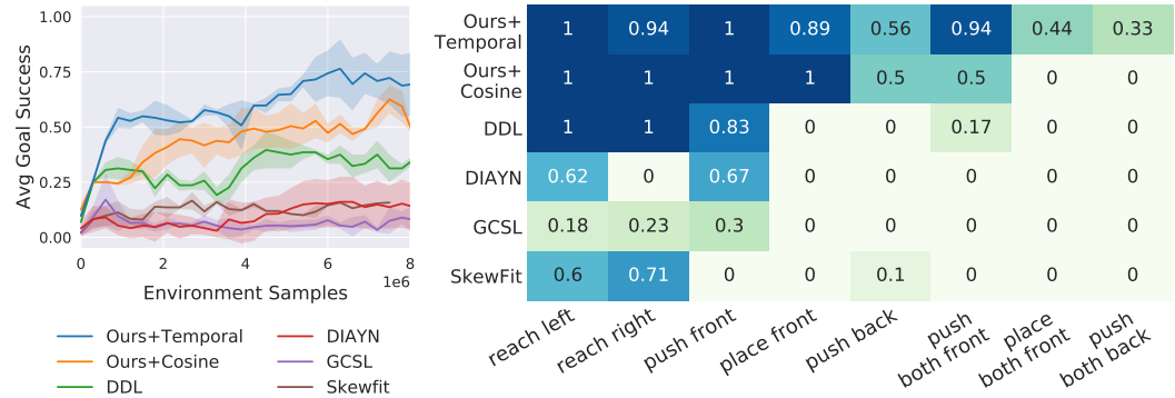
Figure A.4: RoboBin Benchmark . Left: success rates averaged across all 8 tasks. Right: final performance on each specific task. While cosine distance works on simple goals, temporal distance outperforms it on tasks requiring manipulating several blocks (last three columns), as this distance focuses on the part of the environment that's hardest to manipulate. Prior agents only solve the easiest reaching tasks, struggling either with exploration or learning the downstream policy.
