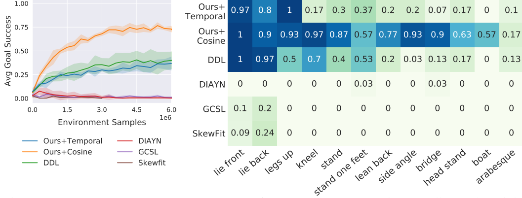
Figure A.2: RoboYoga Walker Benchmark . Left: success rates averaged across all 12 tasks. Right: final performance on each specific task, ranging from light green (0) to dark blue (100%). We observe that the simple latent cosine distance function works well on this task, substantially outperforming other competing agents. In the heatmap, most agents can solve the easy tasks, but only LEXA makes progress on solving a majority of the tasks and achieves good performance.
