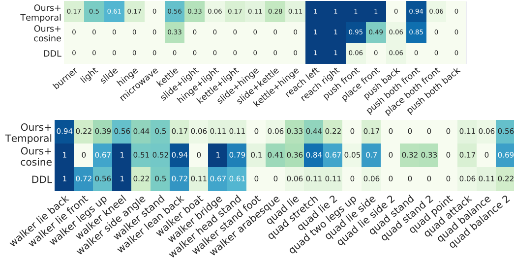
Figure A.6: Single agent trained across Kitchen, RoboBin, Walker, with final performance on each specific task. LEXA with temporal distance is able to make progress on tasks from all environments, while LEXA+cosine and DDL don't make progress on the kitchen tasks.
