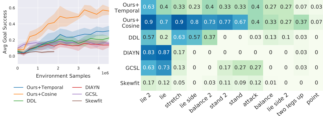
Figure A.3: RoboYoga Quadruped Benchmark . Left: success rates averaged across all 12 tasks. Right: final performance on each specific task, ranging from light green (0) to dark blue (100%). We observe that the simple latent cosine distance function works well on this task, substantially outperforming other competing agents. In the heatmap, most agents can solve the easy tasks, but only LEXA makes progress on solving a majority of the tasks and achieves good performance.
