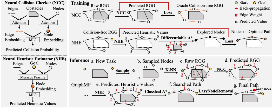
Figure 2: (Left): The architectures of neural collision checker (NCC) and neural heuristic estimator (NHE). The neural collision checker takes a raw RGG and obstacles as input and predicts the collision status of all edges. The neural heuristic estimator takes the collision-free RGG and the goal as input and predicts the heuristic values of all nodes. (Top right): The independent training phases of NCC and NHE. Notice that here we design and utilize a differentiable graph-based A* concatenated to NHE, enabling their joint training in an end-to-end manner. (Bottom right): The main steps of the inference phase to solve the planning task. Once a valid solution is found, we perform the lazy node removal to further reduce the path cost.
