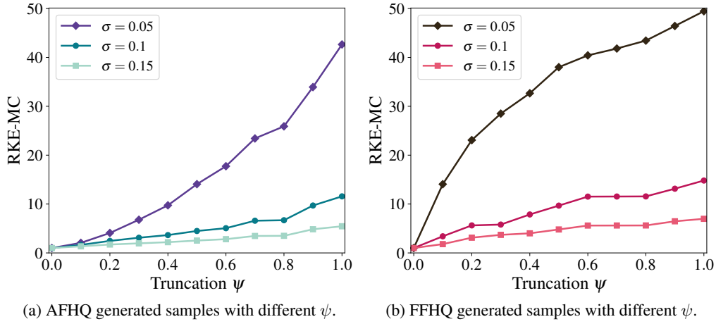
Figure 5: Effect of the bandwidth \sigma on StyleGAN3 with different truncation factor on AFHQ and FFHQ dataset.
