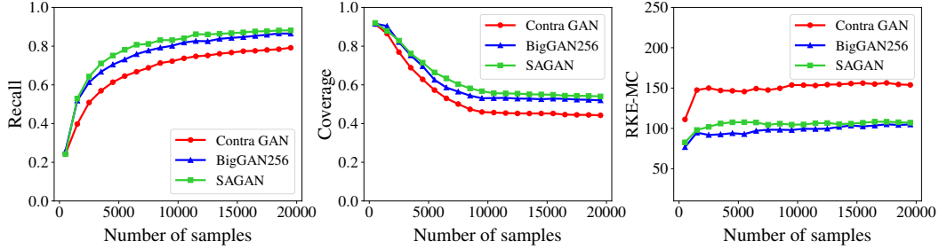
Figure 3: Comparing convergence of Recall, Coverage, and RKE scores on ImageNet dataset.
