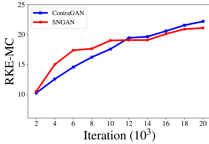
Figure 8: RKE Mode Count during training of ContraGAN and SNGAN on CIFAR10 dataset.
