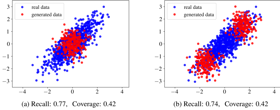
Figure 6: Recall and Coverage can not count the number of modes.
