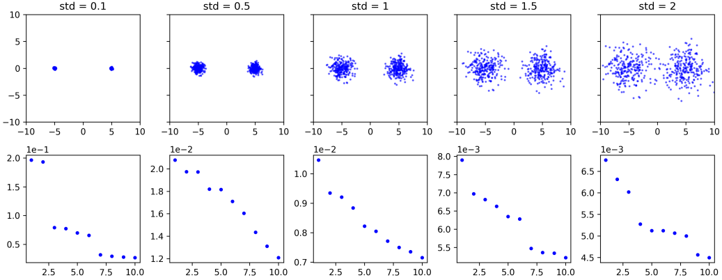
Figure 10: 500 samples from 2D Gaussian distribution with (-5, 0) and (5, 0) as their centers and their eigenvalue in the second row.
