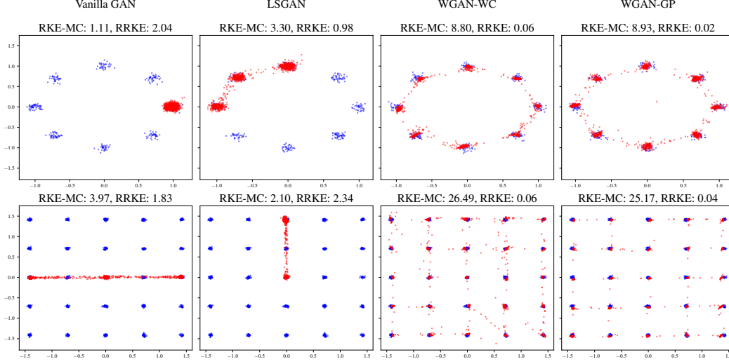
Figure 1: GANs' generated samples for Gaussian mixtures and the RKE-MC ↑ and RRKE ↓ scores.
