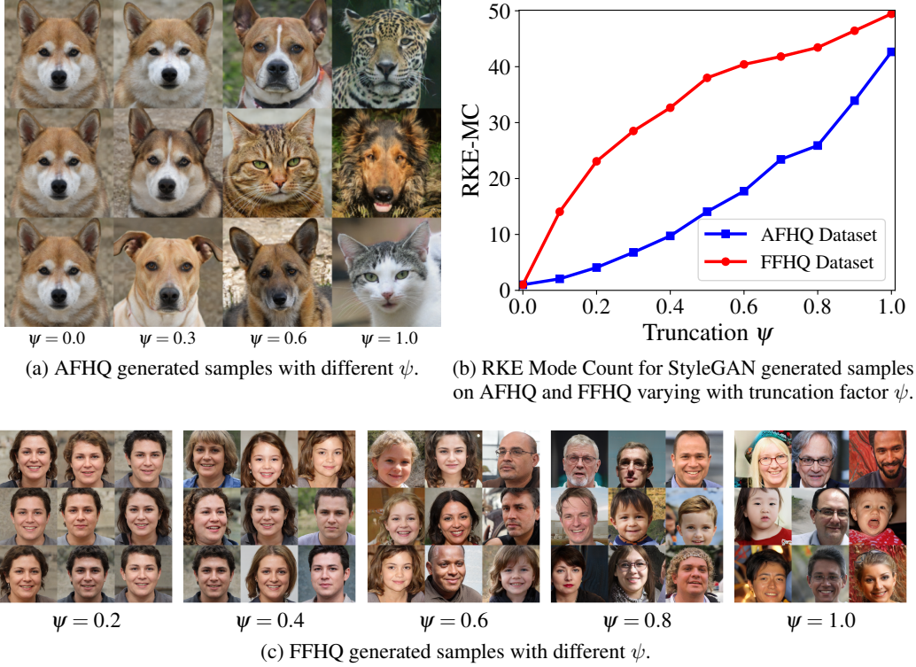
Figure 2: RKE mode count’s behavior under the truncation of the StyleGAN generated samples on AFHQ and FFHQ datasets.
