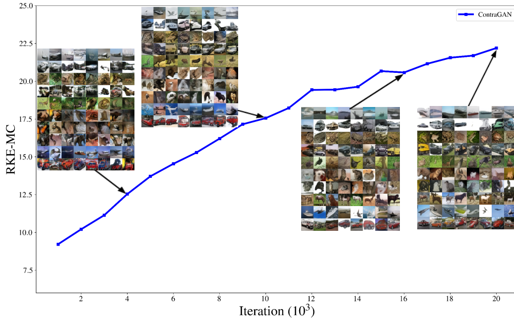
Figure 9: RKE Mode Count during training of Contra-GAN on CIFAR10 dataset with generated samples from 10 classes.
