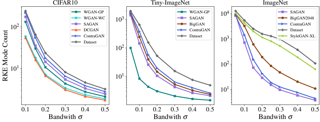
Figure 4: Effect of the bandwidth \sigma on the numerical evaluation
