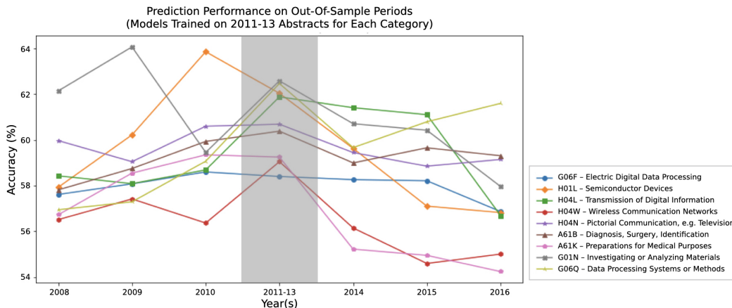
Figure 3: Performance of a BERT decision classifier trained on applications from 2011 to 2013 and evaluated on applications produced in earlier and later years. While model performance decays over time across most categories (suggesting changing acceptance standards), acceptance criteria appear to change more quickly in faster-moving fields (e.g., H01L-Semiconductor Devices and H04W-Wireless Communication) and slower in more developed fields (e.g., A61B-Diagnosis, Surgery, Identification). Of further interest may be the rise in turnover in acceptance criteria in G06Q-Data Processing Systems or Methods starting in 2014, which may coincide with the concurrent growth in development of B2B and fintech products. In future work, it may also be illustrative to use this dataset to investigate the impact of the U.S. Supreme Court decision in Alice Corp. v. CLS Bank International , 573 U.S. 208 (2014), on the software-related patent applications issued after 2014.
