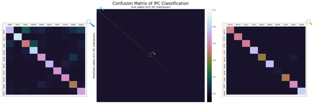
Figure 7: Confusion matrix of IPC code classification at the subclass level. This matrix was obtained from the DistilBERT model that was fine-tuned on the abstract sections. The IPC codes were ordered by their sizes from left to right and from top to bottom, respectively. The light diagonal line present on the center figure represents high recall values. The diagonal line disappears towards the lower right corner, since patents belonging to those IPC subclasses do not appear in our test set.
