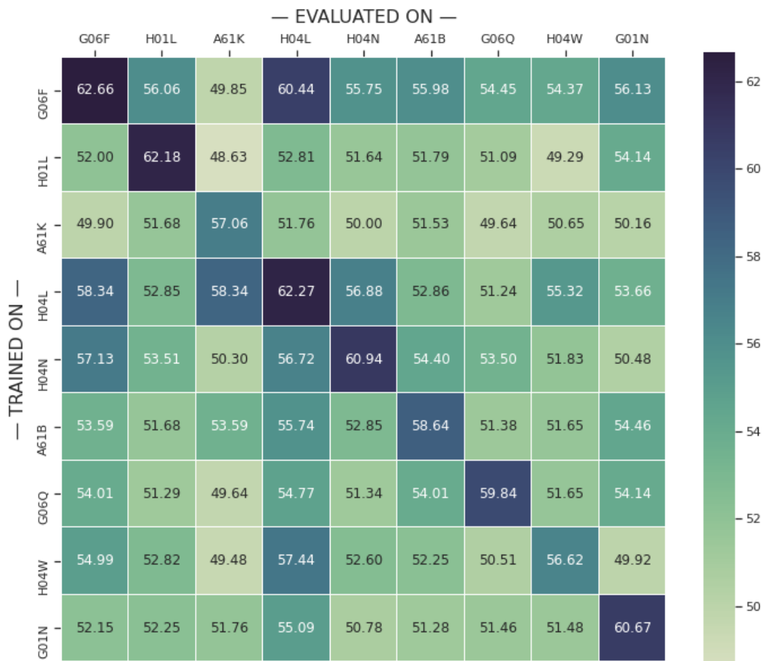
Figure 9: Cross-category evaluation of BERT acceptance prediction classifiers trained on one IPC code evaluated to predict acceptance on other IPC codes. Patent categories that are conceptually similar appear to have closer shared criteria for acceptance (for example, G06F- Electric Digital Data Processing and H04N- Pictorial Communication ). Most models also tend to perform well when evaluated on patent applications in H04L- Transmission of Digital Information ; moreover, the model trained on H04L- Transmission of Digital Information has high predictive power across other application types. This might reflect acceptance criteria in this category involving more high-level evaluations of quality, as opposed to more domain-specific innovations in engineering or manufacturing.
