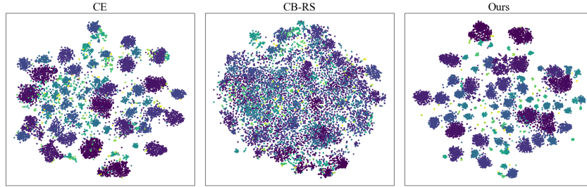
Figure 10: Visualization of learned representation on CIFAR100-LT.
