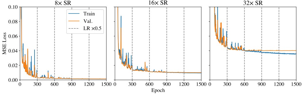
Figure 20: Vanilla RRDB 50.2M MSE loss at 8, 16, and 32 \times SR, with initial learning rate \text{LR} = 1\text{e-}4 .
