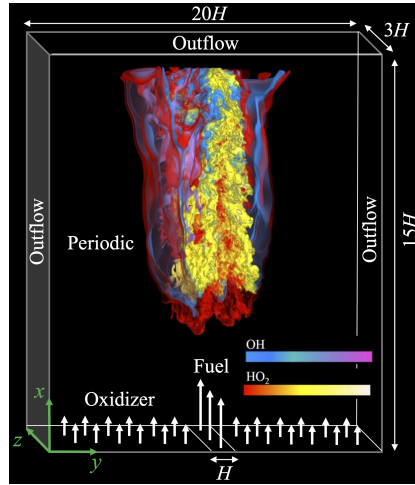
Figure 13: Schematic of the DNS of slot-burner setup. The contours correspond to OH and \text{HO}_2 species. Reprinted from [27], Copyright 2021, with permission from Elsevier.
