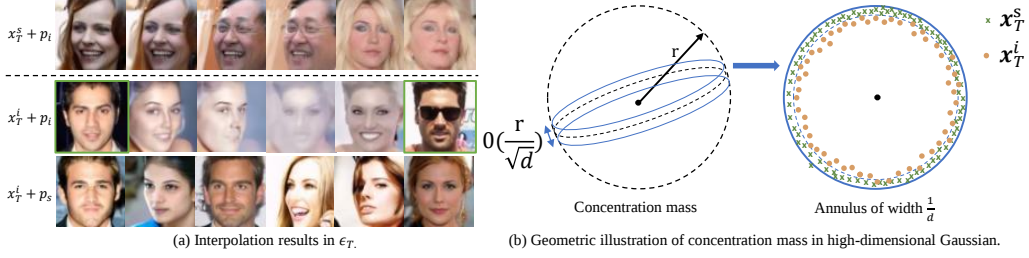
Figure 2: Illustration of distance effect from the qualitative results and geometric properties. (a) The interpolation are conducted on CelabA-64, with different combinations for latent encoding sources and sampling methods. Following the same denoising process p_i , inverted latent encodings lead to distorted images. (b) The inversion process reverses images to the latent encodings at the area of less concentration mass with a smaller radius. \mathcal{O}(\frac{r}{\sqrt{d}}) is the width of the slice for the concentration mass.
