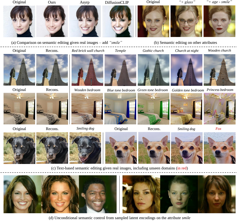
Figure 1: We present the BoundaryDiffusion for efficient ( single-step ), effective and light-weight semantic control on multiple application scenarios with frozen pre-trained DDMs. Different from existing works, our BoundaryDiffusion is a learning-free method that achieves SOTA performance without learning any extra networks, in contrast to e.g. Asyrp [35], which requires training auxiliary editing neural networks, and DiffusionCLIP [31], which fine-tunes the pre-trained DDMs. We include more randomly selected non-cherry-picked results in Appendix G as qualitative demonstrations.
